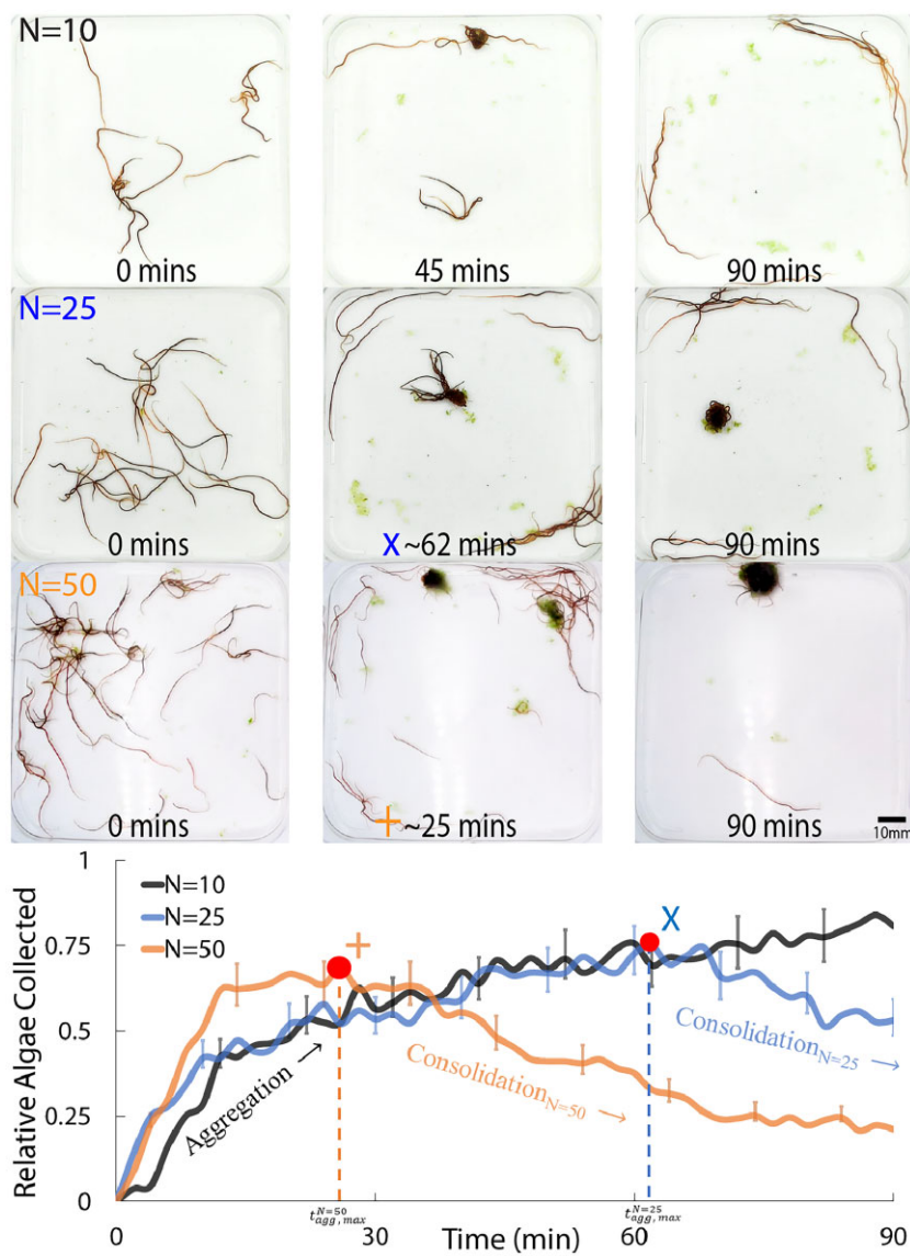
Fig. 2 Collective-gathering of algae by blackworms. (Top) Three blackworm trials with N = 10, 25, and 50 worms collecting 10 mg of algae. The maximum aggregation period for N = 25 and 50 are labeled in the graph below. (Bottom) Graph showing the relative algae collected for the three populations over time. The data were obtained by thresholding algae in ImageJ. Each curve represents the average relative algae collected, and the vertical bars show the standard error for n = 5 trials. (Supplementary Movie 1).
