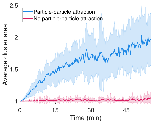
Fig. 6 Gathering efficiency in the active polymer model. The collecting–gathering efficiency of the active polymer worm is quantified by the average area of particle clusters as a function of time, normalized by the area of 1 particle, for the model without particle-particle attraction (pink) and with particle-particle attraction \varepsilon_{pp} = 1 (blue). The worm-particle interaction strength is \varepsilon_{wp} = 2 . An average of over 20 simulations is shown for each case, with the shaded regions representing one standard deviation.
